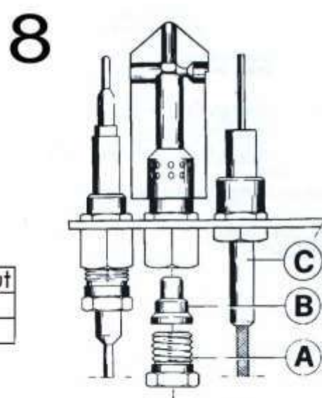
pilot burner
